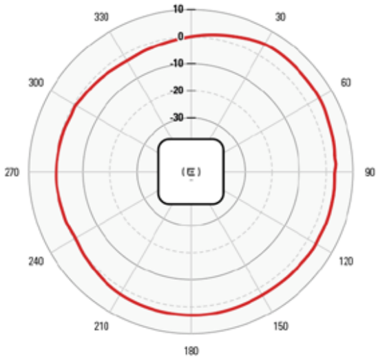
AZIMUTH 2.4 GHZ
