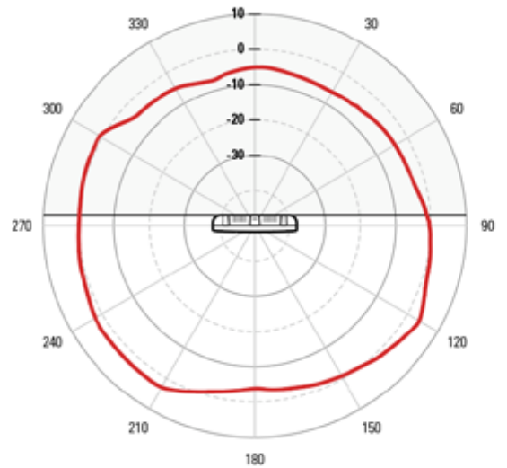
ELEVATION 5 GHZ
