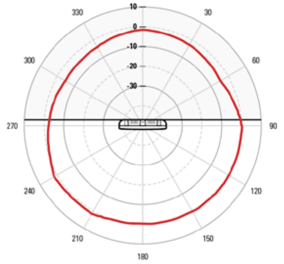
ELEVATION 2.4 GHZ
