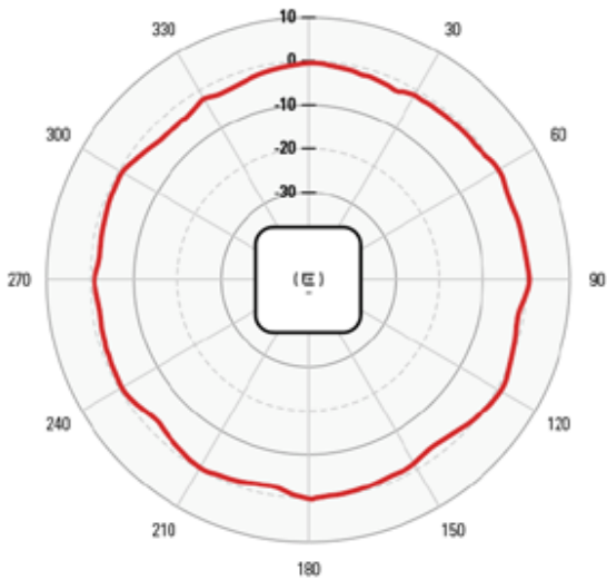
AZIMUTH 5 GHZ
